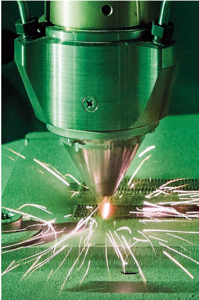
Image 5: 3D metal printing in record time: The CNC machine modified for the EHLA process can move tools in a fast, highly dynamic and precise manner in a lateral direction. With a rotary and tilting table, it is suitable not only for additive manufacturing, but also for free-form surface coatings. © Fraunhofer ILT, Aachen, Germany.
