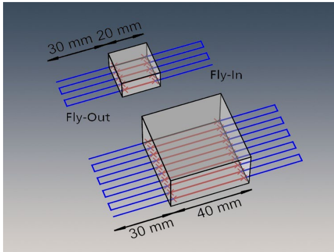
Image 3: High dynamics: With EHLA 3D, productivity sinks and swims with the interaction of fly-in and fly-out. © Fraunhofer ILT, Aachen, Germany.
